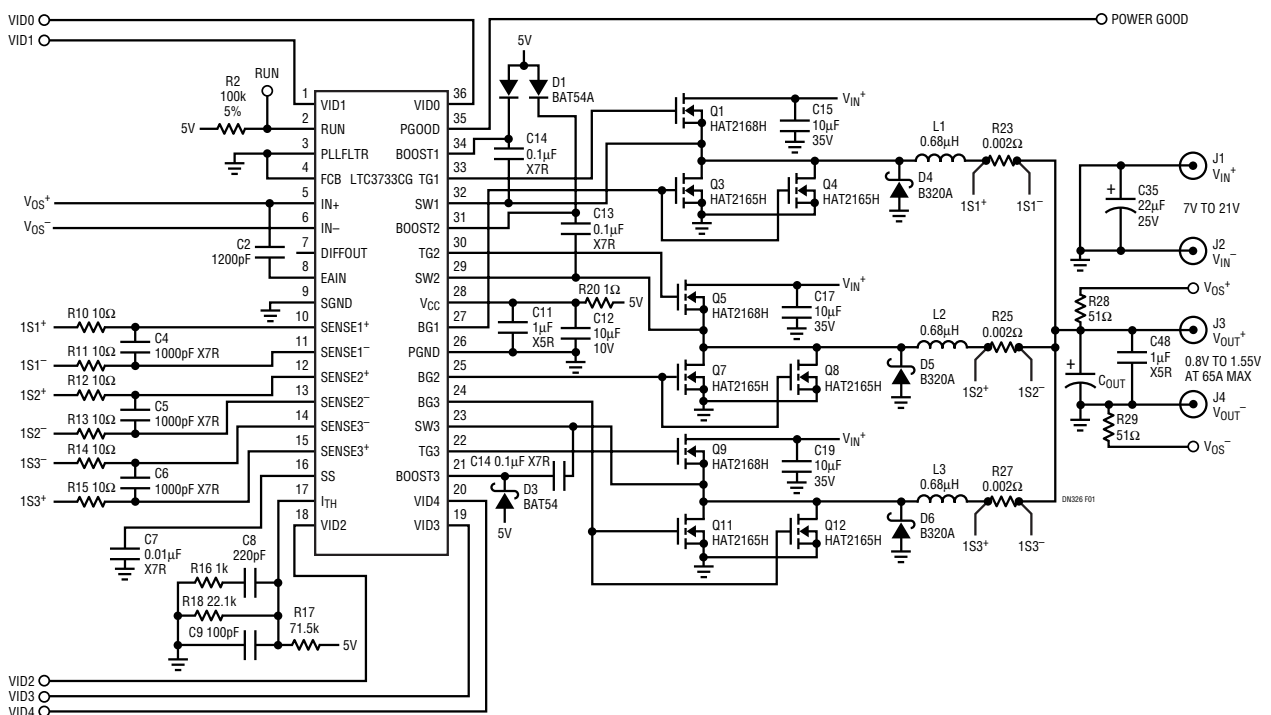
Figure 1. 65A AMD Processor Power Supply Using the LTC3733
