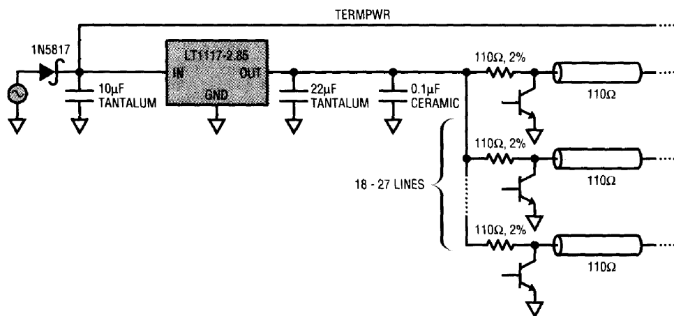
Figure 3. Active Termination
