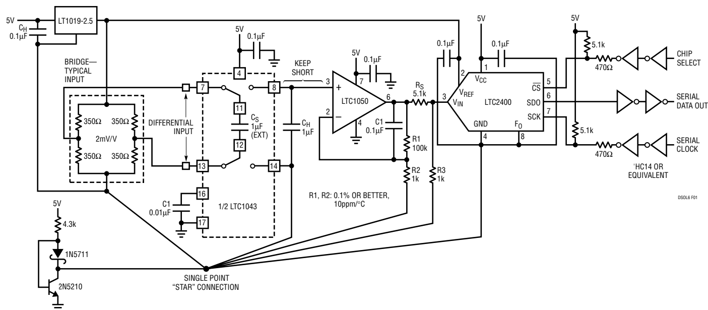
Figure 1. Single Supply Differential to Single-Ended Converter for Low Level Inputs with "Live at Zero" Operation
