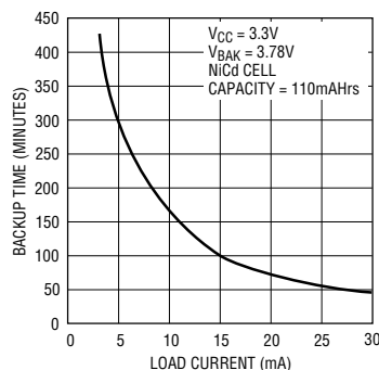
Backup Time vs 3.3V Output Load Current
