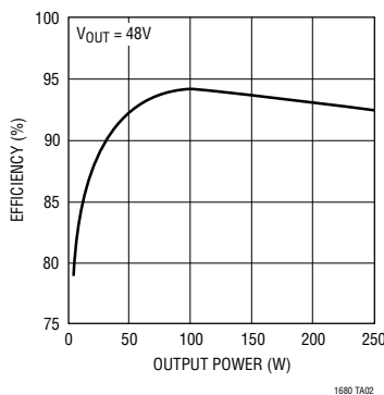
Efficiency vs Output Power
