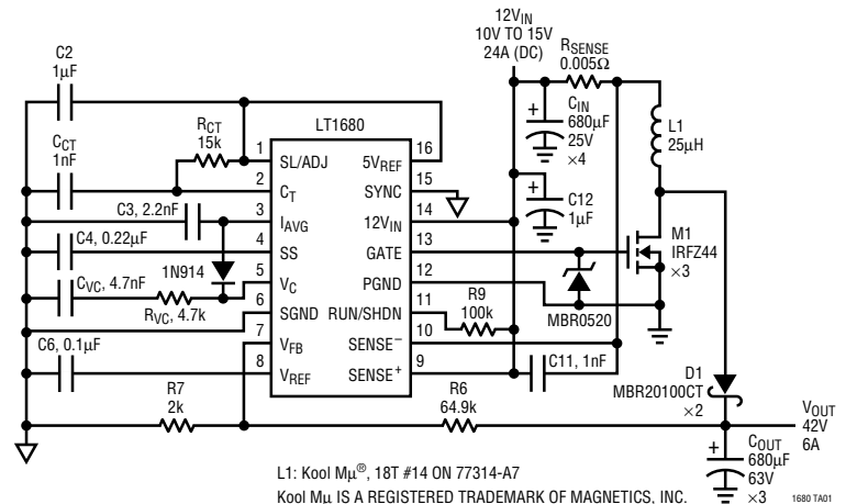
12V to 42V, 250W Boost
