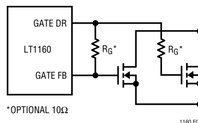
Figure 1. Paralleling MOSFETs
