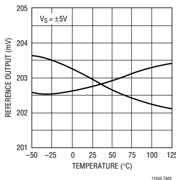
Figure 2. Reference Output vs Temperature of Two Typical Units
