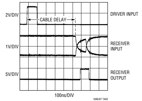
Figure 2. Novel Architecture of LTC1686/LTC1687 Full-Duplex Transceivers Maintain a Very Tight Propagation Delay Window for Both the Receiver and the Driver. Here is a 10Mbps Data Pulse Delay Over 400 Feet of Category 5 UTP
