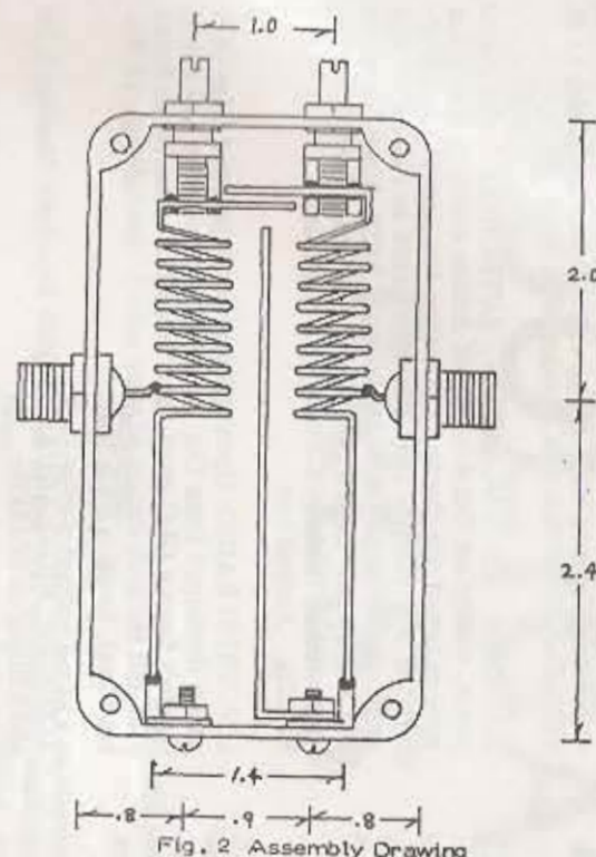
Fig. 2 Assembly Drawing
