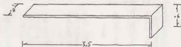
Fig. 3 Shield detail
