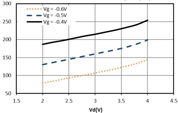
AMM-6702UC Quiescent Current Consumption (mA) vs. Vd
