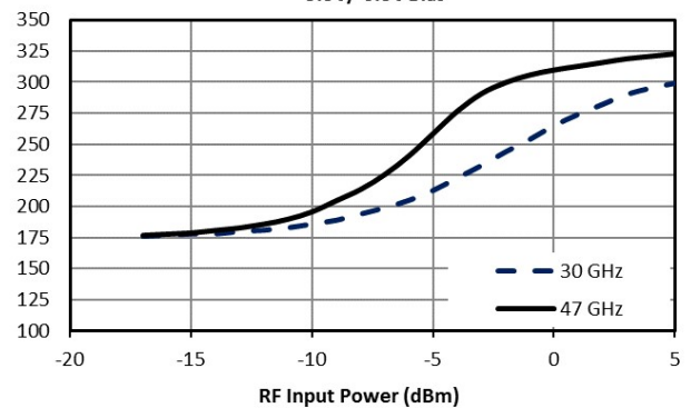
AMM-6702UC Current Consumption (mA) vs. RF Input Power, 3.5V/-0.5V Bias
