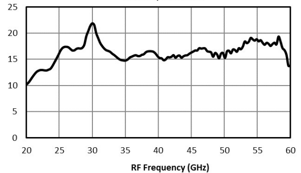
Input IP3 of Marki MMIQ-1865L Mixer using AMM-6702UC as LO Driver Amplifier (dBm), 3.5V/-0.4V Bias Condition, 3dBm Input, IF = 100 MHz, LO = RF - IF
