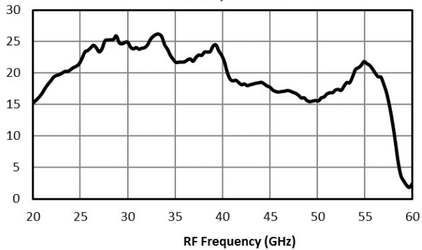
Input IP3 of Marki MMIQ-1865H Mixer using AMM-6702UC as LO Driver Amplifier (dBm), 3.5V/-0.4V Bias Condition, 3dBm Input, IF = 100 MHz, LO = RF - IF
