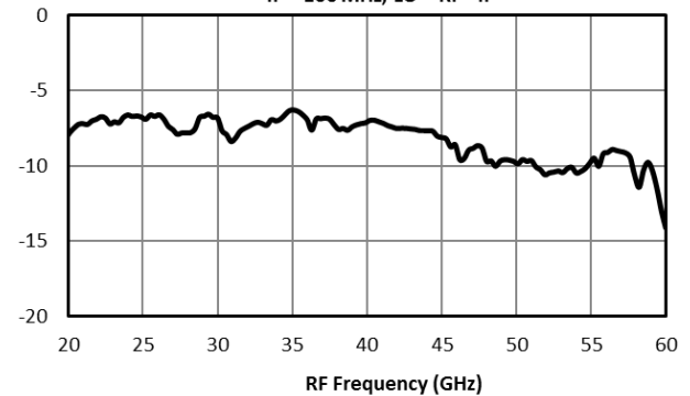
Conversion Loss of Marki MMIQ-1865L Mixer using AMM-6702UC as LO Driver Amplifier (dB), 3.5V/-0.4V Bias Condition, 3dBm Input, IF = 100 MHz, LO = RF - IF
