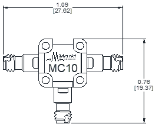
Topside View
