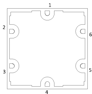
X-RAY VIEW CSP PACKAGE
