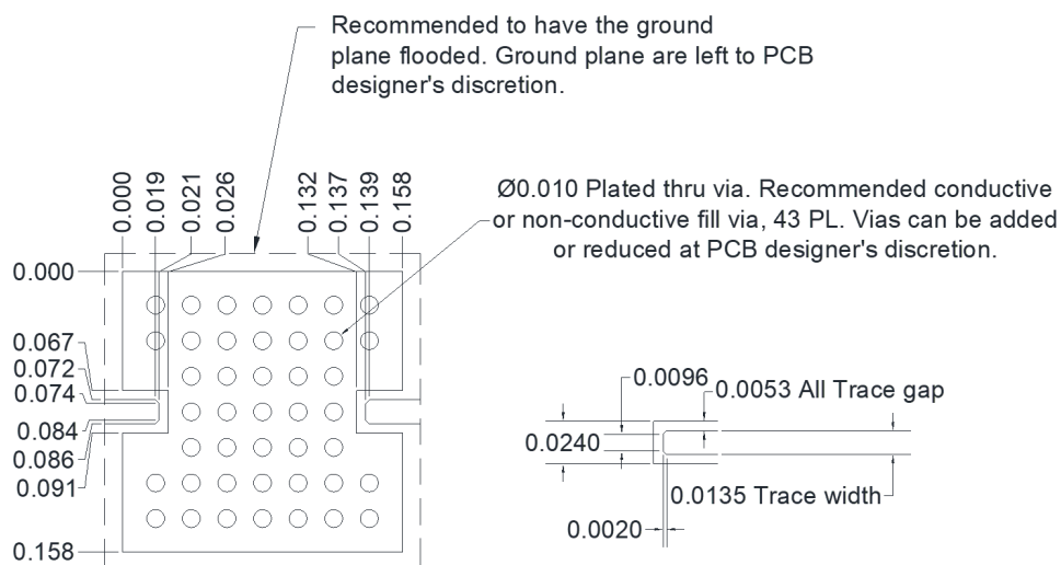
QFN 4mm Sample Drawing X-Ray view
