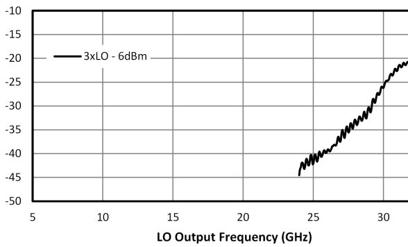
Odd LO Harmonic to RF Leakage (dBm)
