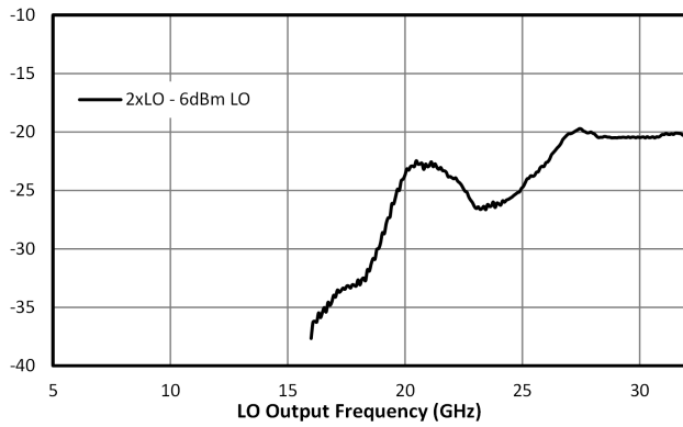
Odd LO Harmonic to RF Leakage (dBm)
