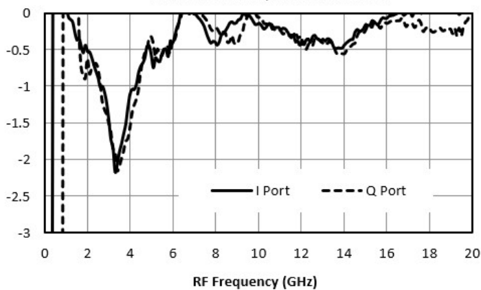
Vector Modulator Insertion Loss (dB)
