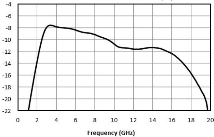
Vector Modulator Insertion Loss (dB)
