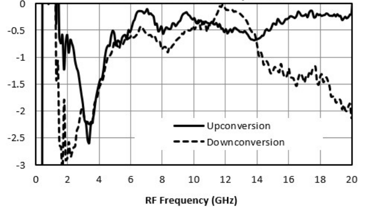
Upconversion Conversion Loss Compression (dB) 23 dBm LO Power, 13 dBm IF Power
