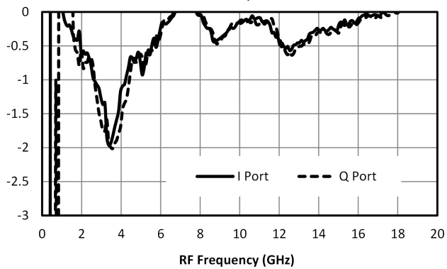
Vector Modulator Insertion Loss (dB)
