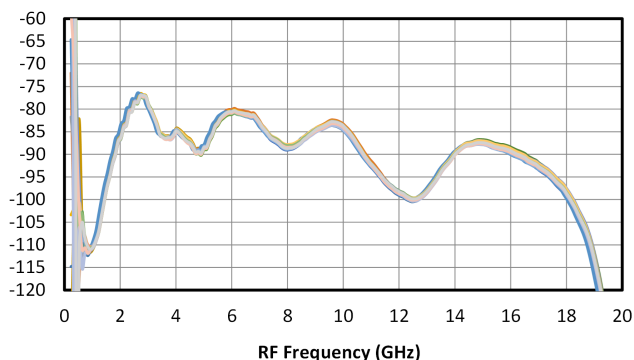
L-R Isolation Variation (dB) 20 Units
