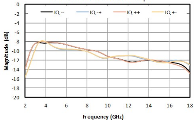
Vector Mod Insertion Loss +3dBm Input
