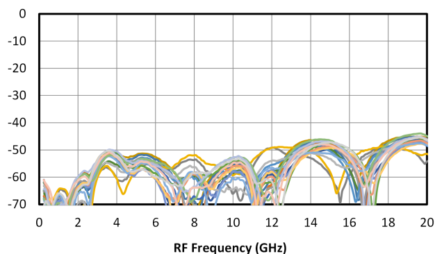
L-R Isolation Variation (dB) 20 Units
