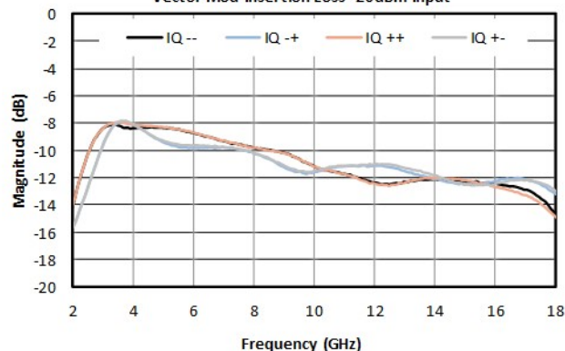
Vector Mod Insertion Loss -20dBm Input
