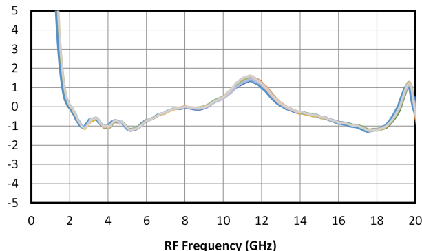
Amplitude Balance Variation (dB) 20 units
