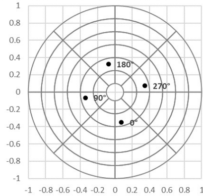
Vector Modulator Insertion Loss vs Phase: 10GHz (dB)
