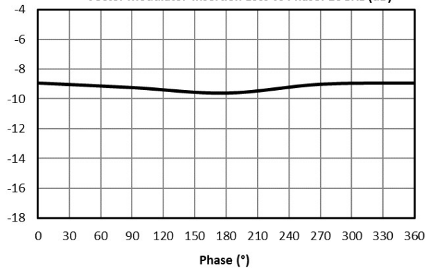
Vector Modulator Insertion Loss vs Phase: 10GHz (dB)
