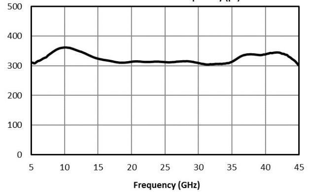
Vector Modulator Group Delay (ps)
