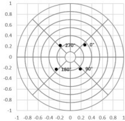
Vector Modulator Insertion Loss vs Phase: 20GHz (dB)
