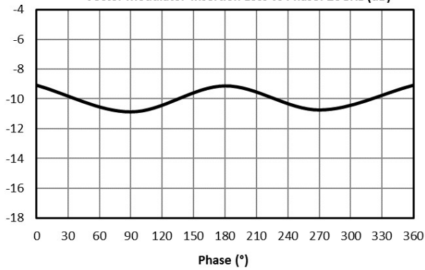
Vector Modulator Insertion Loss vs Phase: 20GHz (dB)
