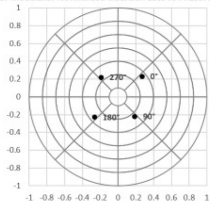
Vector Modulator Normalized Insertion Loss vs Phase: 20GHz (U)
