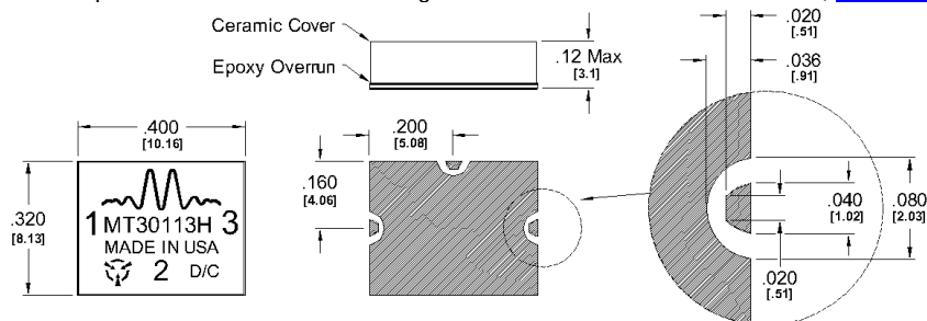
Outline Drawing – CQG-2 Package
