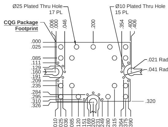
CQG-Package Landing Pattern
