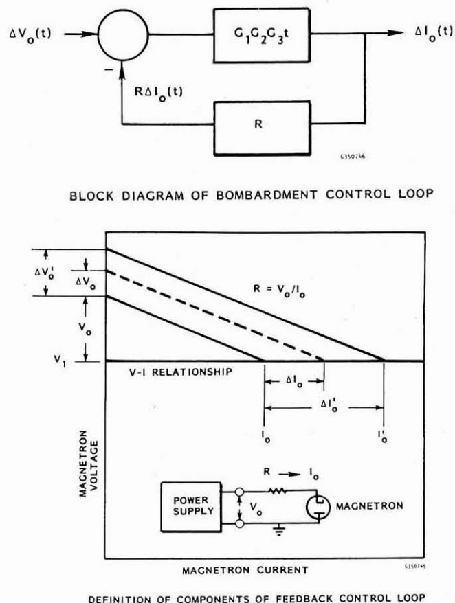
Figure 4. Control theory format for the transient and steady state behavior of the magnetron.
