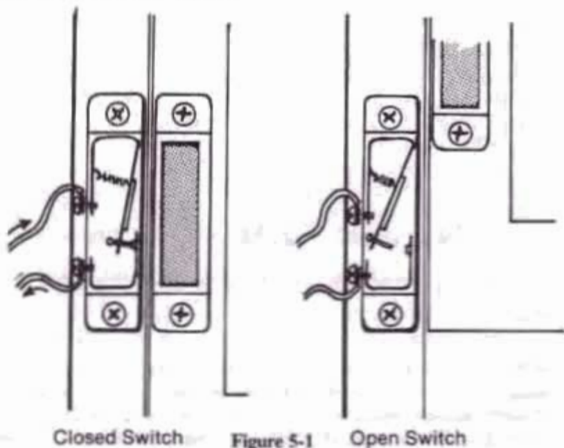
A common magnetic switch. On the left, the circuit is closed. When the magnet is removed (right), the circuit opens and triggers the alarm.
