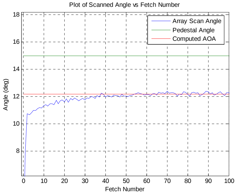
Figure 109. Plot of Angle against Fetch Number for AOA of 15°
