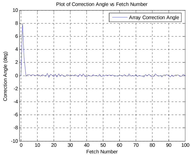
Figure 110. Plot of Correction Angle against Fetch Number for AOA of 15°
