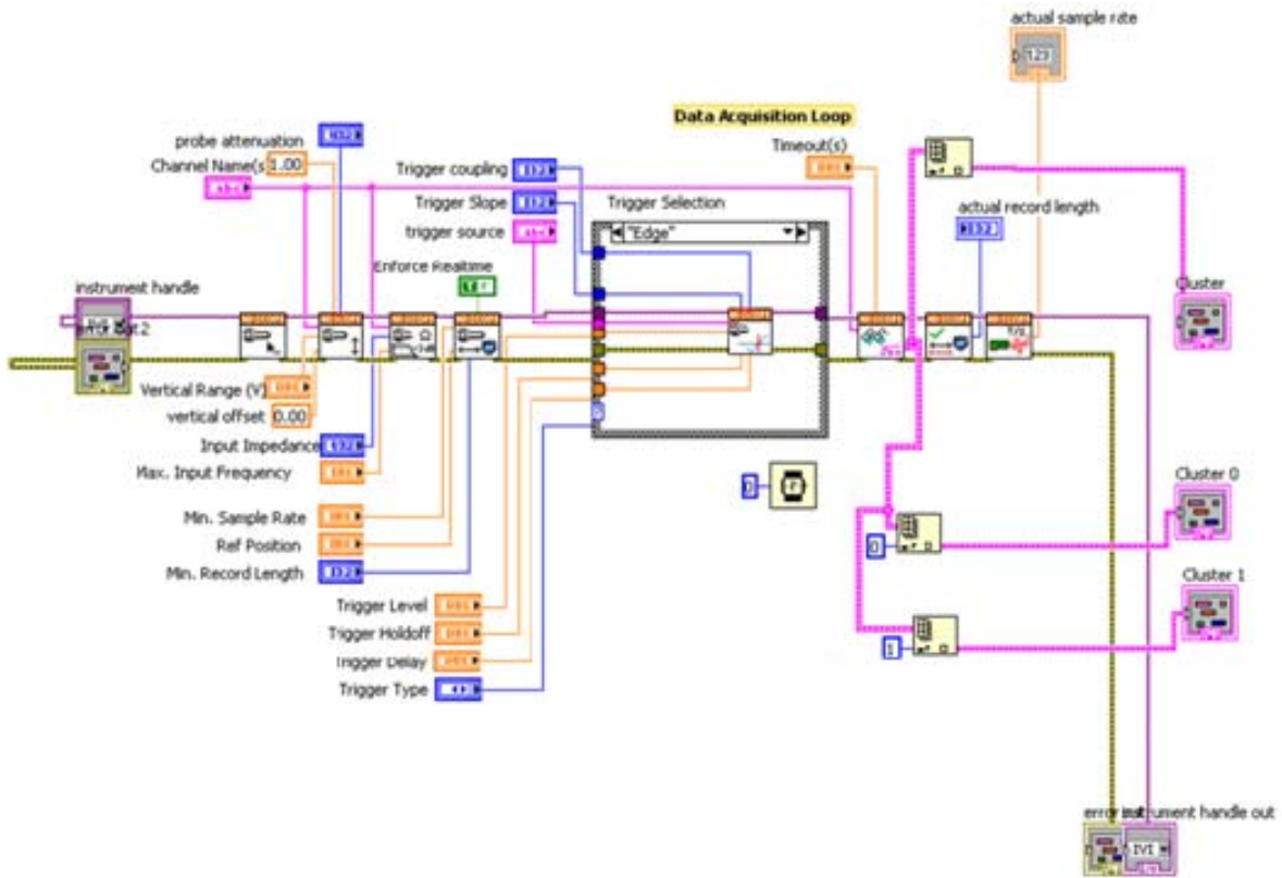
Figure 33. Open and Fetch from 5112 sub VI
