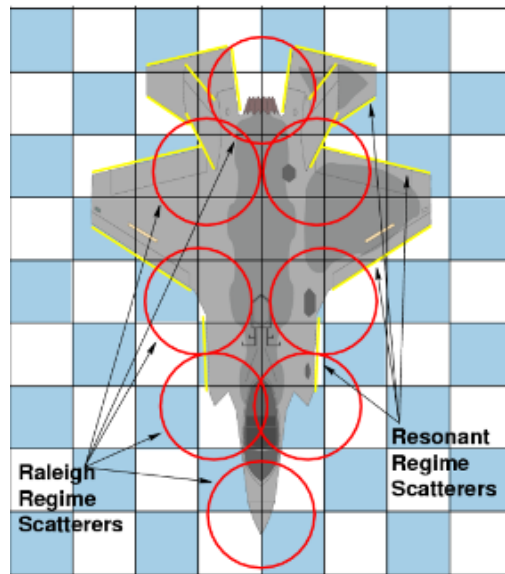
Figure 73. F-35 JSF in the 2 Metre Band VHF (150 MHz) Radar (From [107])
