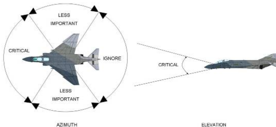
Figure 33. RF RCS Importance According to the Expected Threat Angles (After [39])
