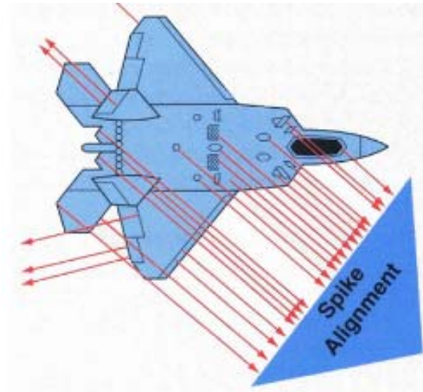
Figure 35. F-22 Raptor's RCS Reduction Technique by Shaping (From [49])
