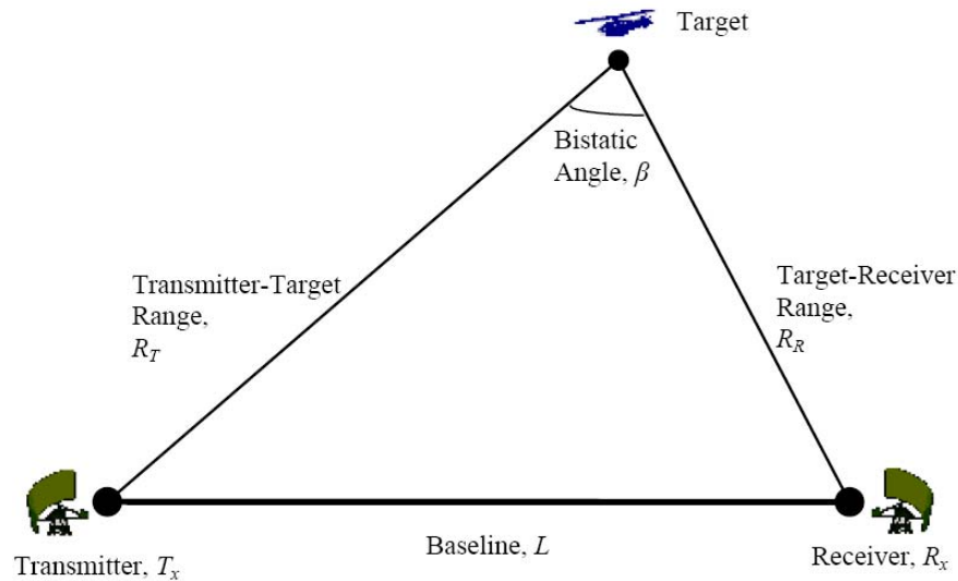
Figure 82. Bistatic Radar Configuration (From [111])
