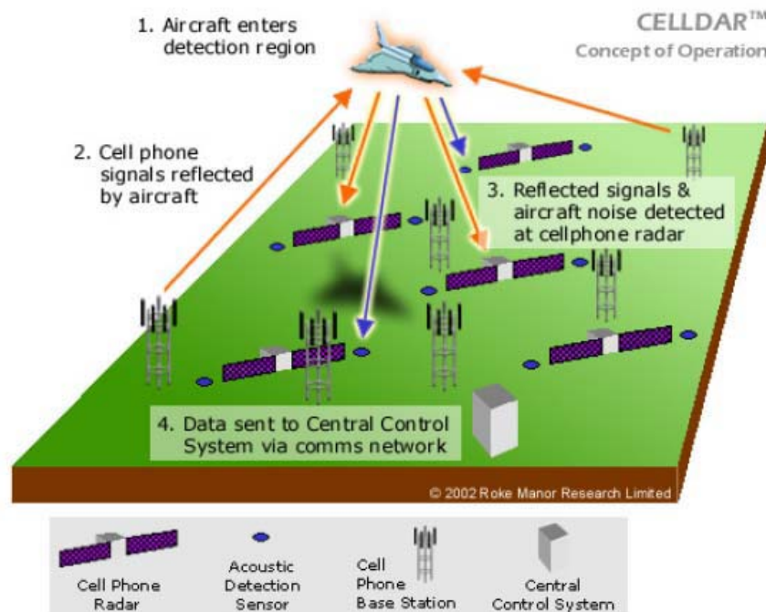
Figure 85. BAe System's Celldar Passive Radar Network Based on Cell Phone Signals (From [117])
