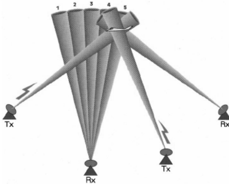
Figure 83. Multistatic Radar Configuration (From [114])
