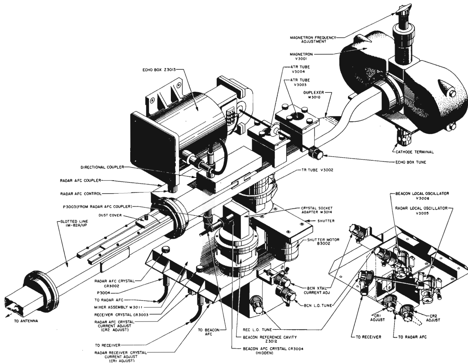
Figure 10-9.—R-f section of receiver-transmitter in AN/SPS-10D. 32.180
