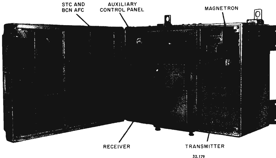
Figure 10-8.—Receiver-transmitter.
