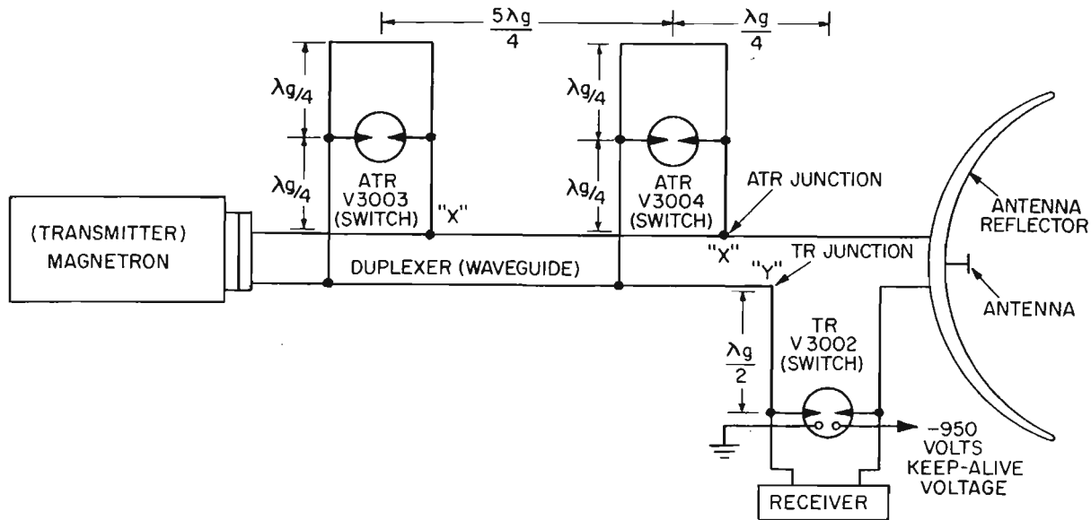
Figure 10-12.—Duplexer (microwave switching). 32.183
