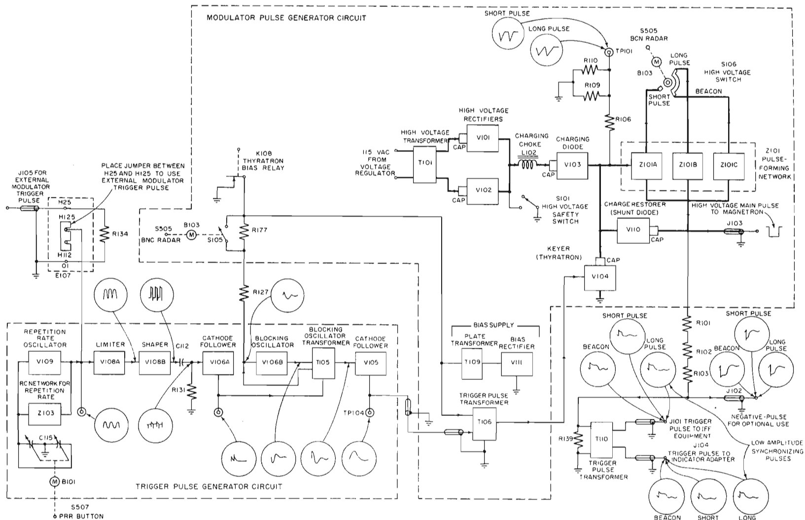
Figure 10-5.—Modulator, block diagram.
