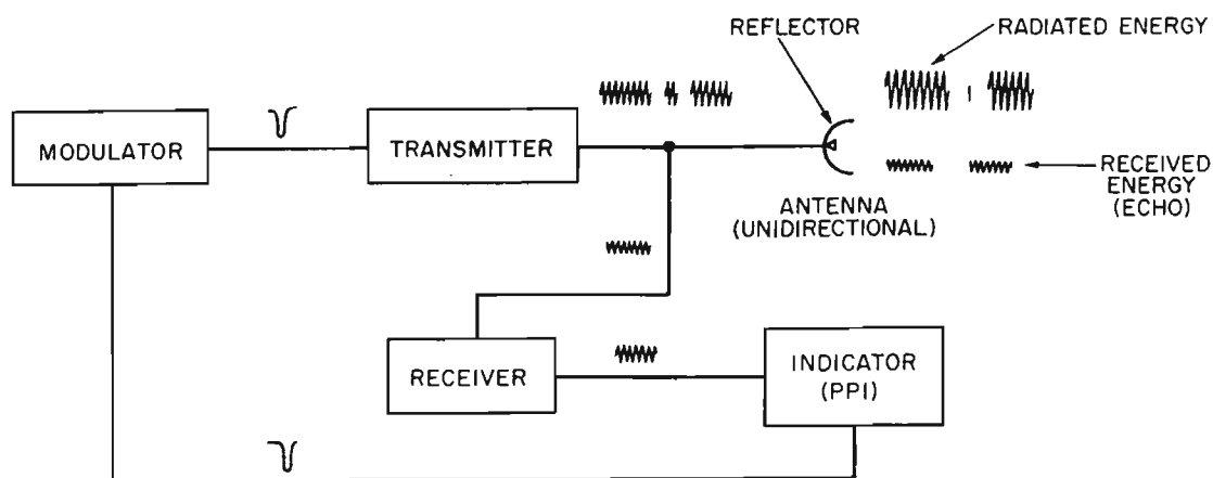
Figure 10-2.—Radar Set, AN/SPS-10D, functional diagram.
