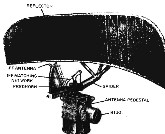
Figure 10-15.—Antenna assembly.
