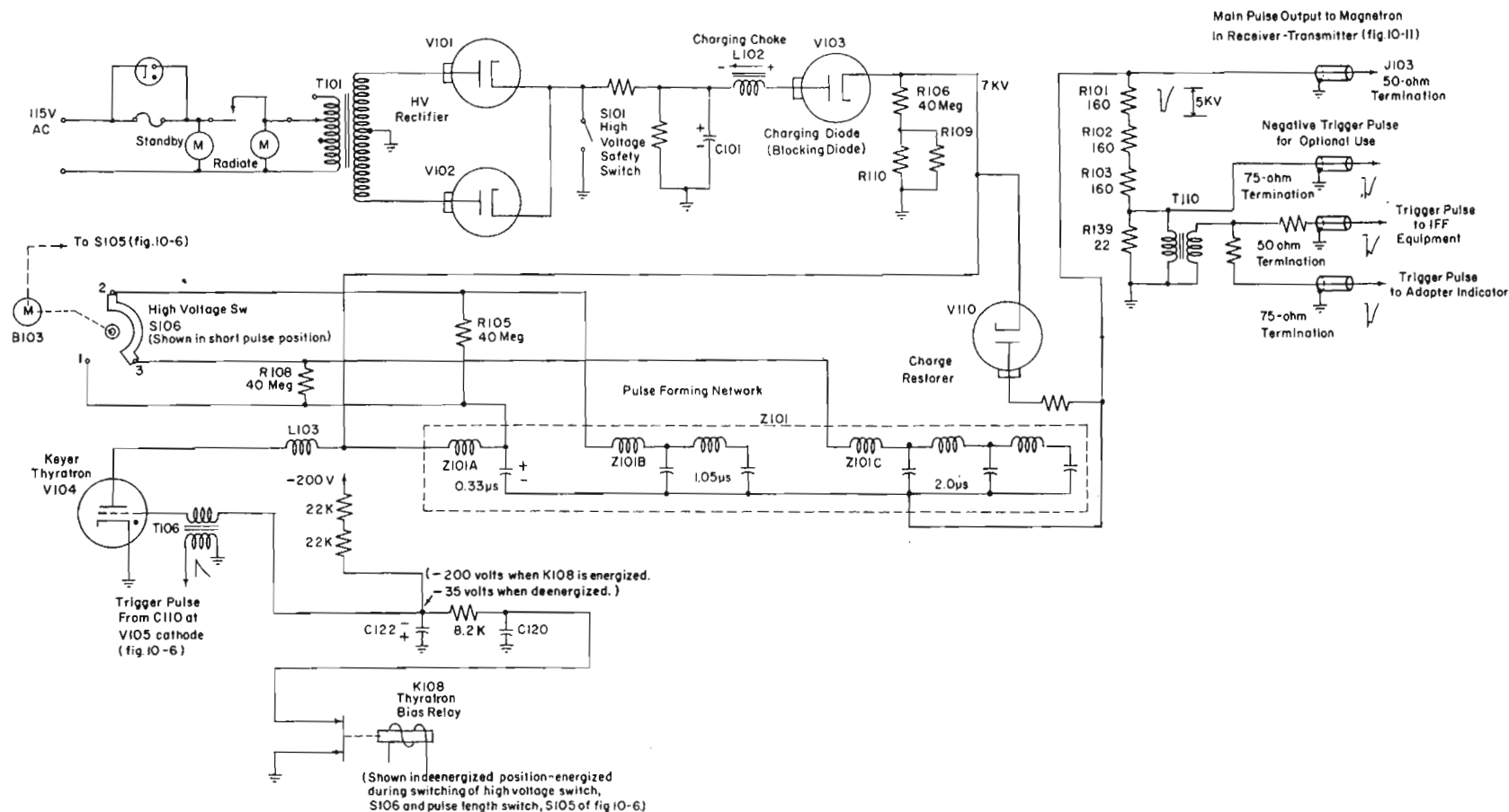
Figure 10-7.—Pulsing circuit and pulse network.
