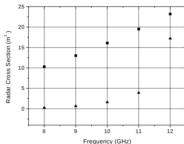
Figure 12. Attenuation values ( \text{m}^2 ) as a function of frequency of RAM with dielectric component. ■ - reference, ▲ - PAni loaded panel.
