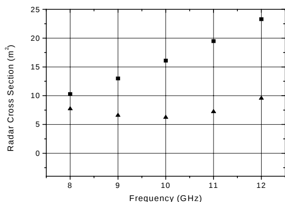
Figure 10. Attenuation values ( \text{m}^2 ) as a function of frequency of RAM loaded with magnetic fillers. ■ - reference, ▲ - painted panel.
