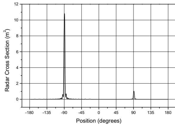
Figure 6. RCS measurements (in m^2 ) for the panel (20 cm x 17 cm) at 8 GHz. Reference side ( -180^\circ to 0^\circ ) and RAM (magnetic component) side ( 0^\circ to +180^\circ ).
