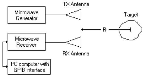
Figure 2. RCS measurement setup.
