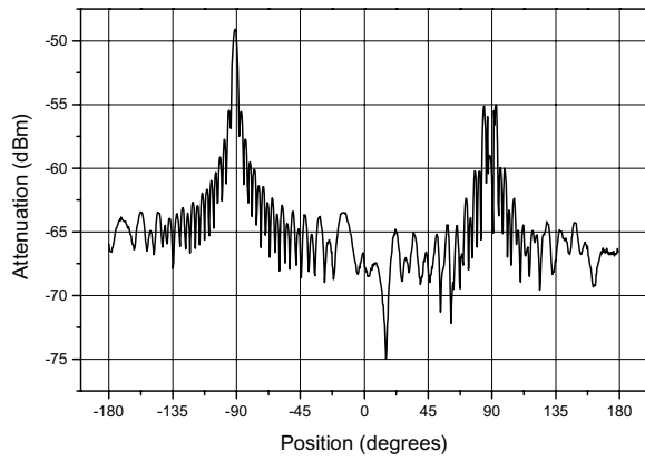
Figure 5. RCS measurements (in dBm) for the panel (20 cm x 17 cm) at 8 GHz. Reference side ( -180^\circ to 0^\circ ) and RAM (magnetic component) side ( 0^\circ to +180^\circ ).
