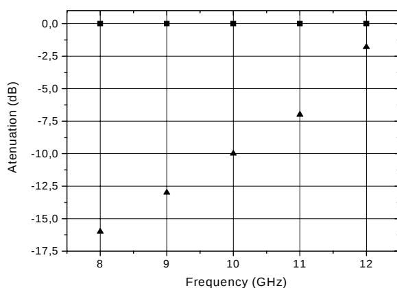
Figure 11. Attenuation values (dB) as a function of frequency of RAM with dielectric component. ■ - reference, ▲ - PAni loaded panel.
