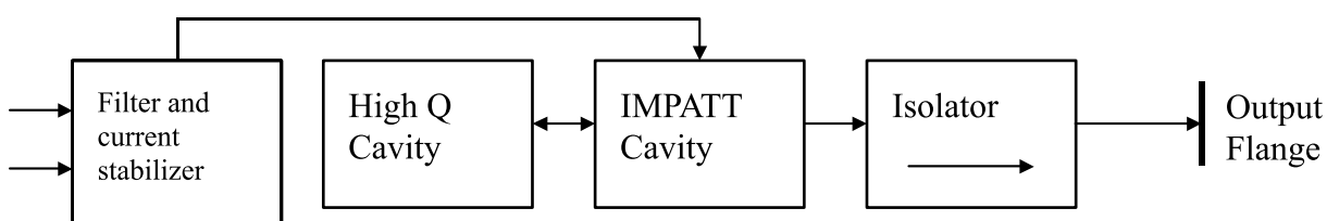
Scheme of oscillator
