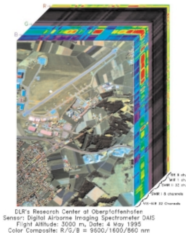
Fig. 28. Colour composite image recorded using the digital airborne imaging spectroradiometer (permission from German Aerospace Centre DLR).
