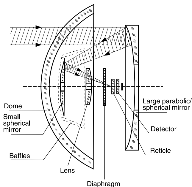
Fig. 7. Optical diagram of a typical passive non-imaging seeker.
