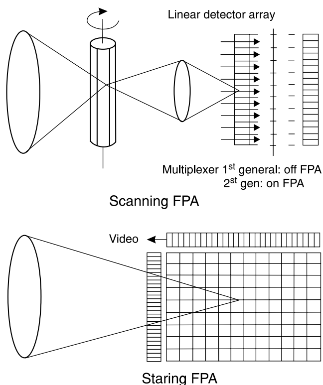
Fig. 14. Scanning (a) and staring (b) focal plane arrays.
