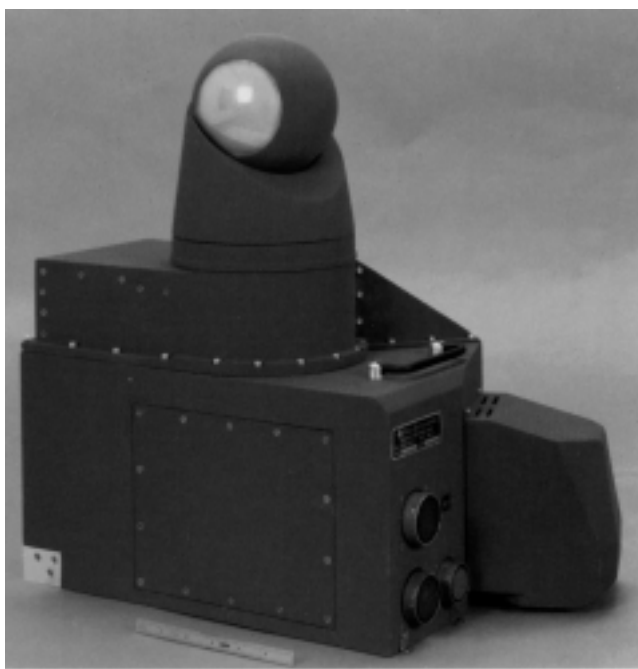
Fig. 22. Falcon Eye, a representative conformal FLIR (after Ref. 18).
