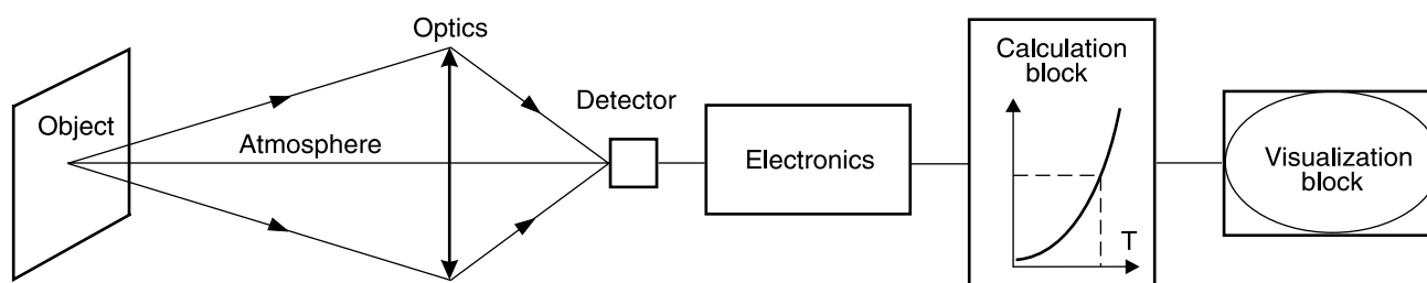
Fig. 24. General diagram of a simple non-contact thermometer (after Ref. 19).
