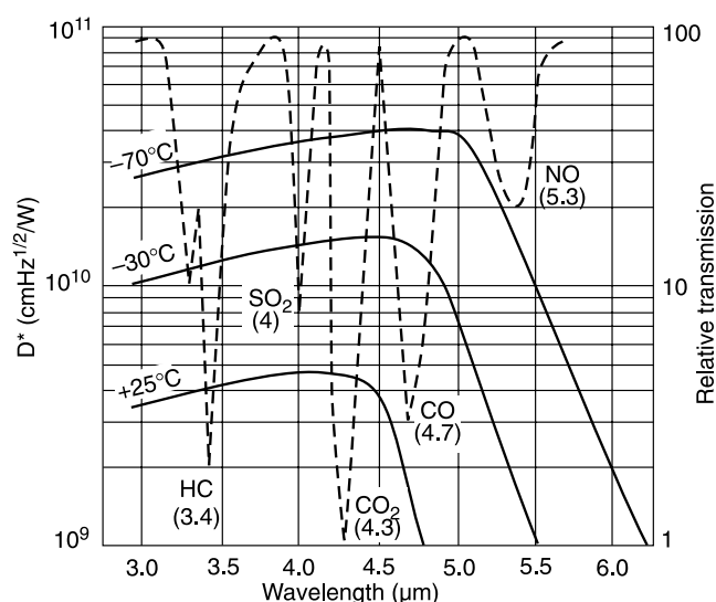
Fig. 31. Detectivity of lead selenide detectors as a function of wavelength at operating temperatures of +25°C, -30°C and -70°C, along with absorption spectra of same common air pollutants.
