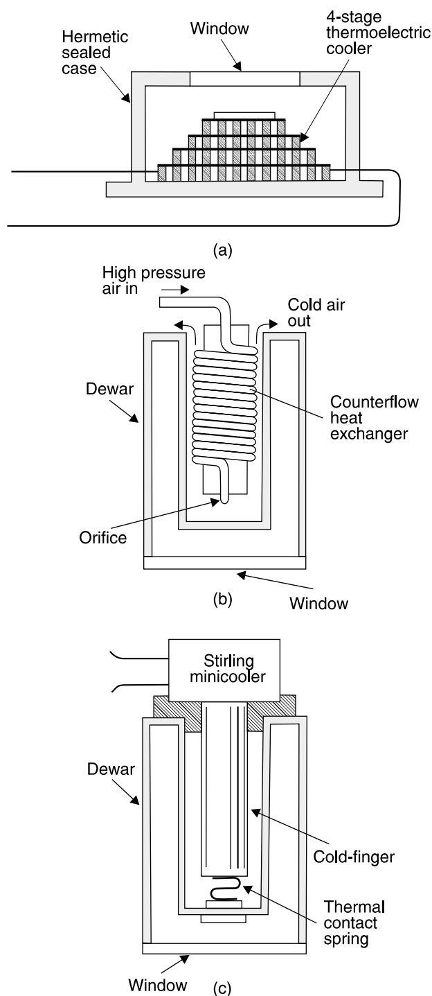
Fig. 4. Three ways of cooling IR detectors: (a) four-stage thermoelectric cooler (Peltier effect), (b) Joule-Thompson cooler, and (c) Stirling-cycle engine.
