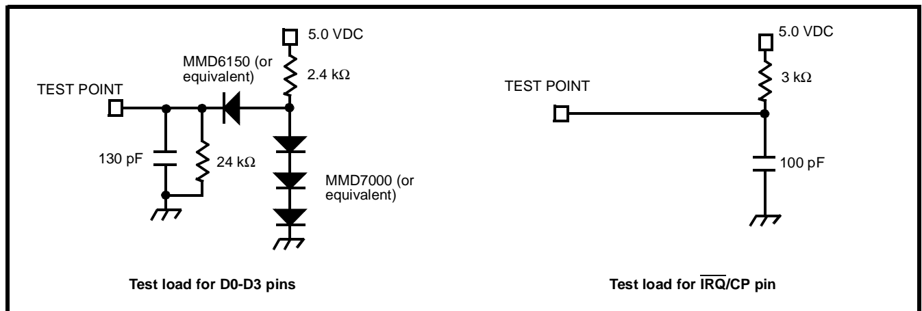
Figure 14 - Test Circuits
