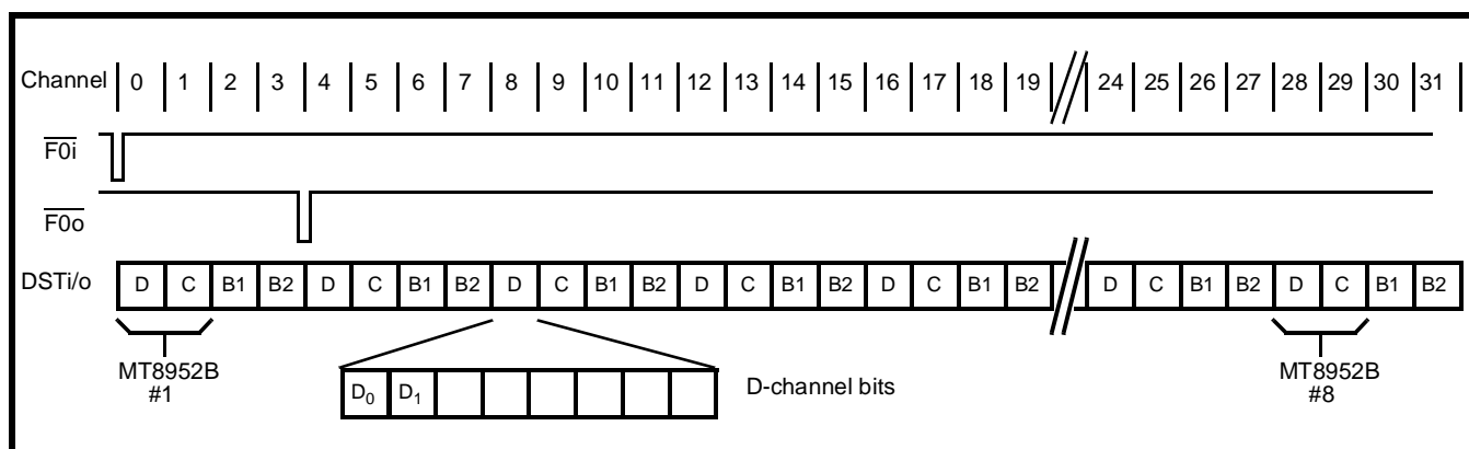
Figure 9 - Composite ST-BUS Frame For Example 3.1
