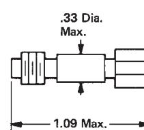
Model 61B SMA-F to SMA-M
