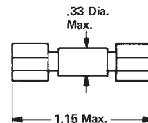
Model 70 3.5mm-M to 3.5mm-M
