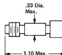
Model 71 3.5mm-F to 3.5mm-M
