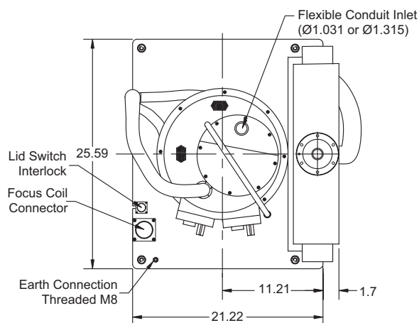
Top View of Trolley Assembly
