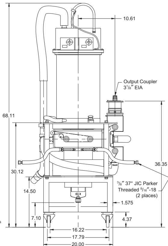
Front View of Trolley Assembly
