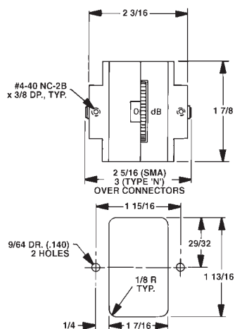
TYPICAL PANEL CUTOUT SINGLE*
