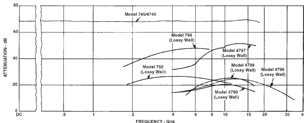
Figure 2. Attenuation vs. Frequency of Variable Attenuators
