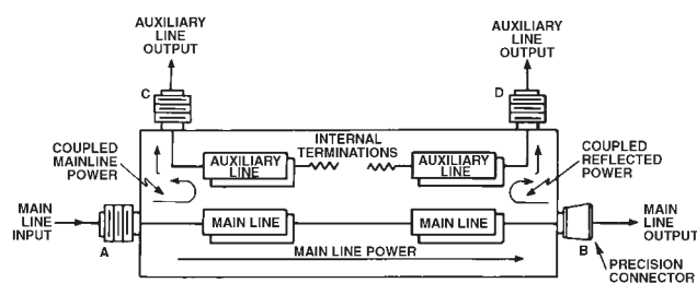
Figure 10. Dual Coaxial Directional Coupler
