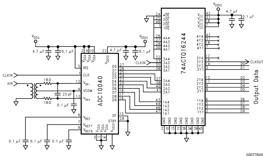
FIGURE 5. A Simple Application Using a Differential Driving Source
