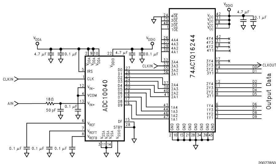
FIGURE 6. A Simple Application Using a Single Ended Driving Source
