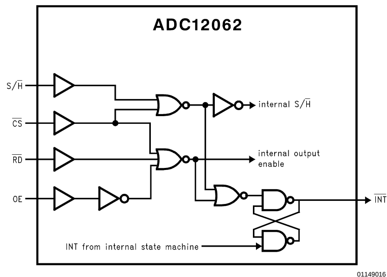
FIGURE 6. ADC Control Logic
