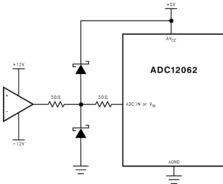
FIGURE 9. Input Protection
