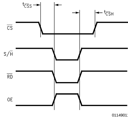
FIGURE 3. \overline{\text{CS}} Setup and Hold Timing for S/H, \overline{\text{RD}} , and OE
