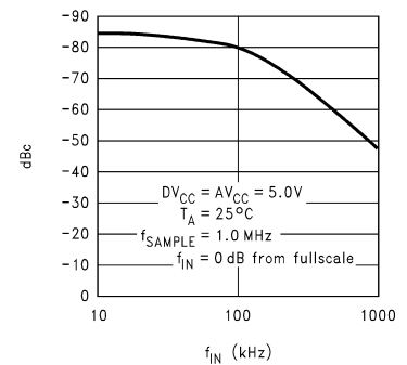
THD vs Input Frequency (ADC IN)
