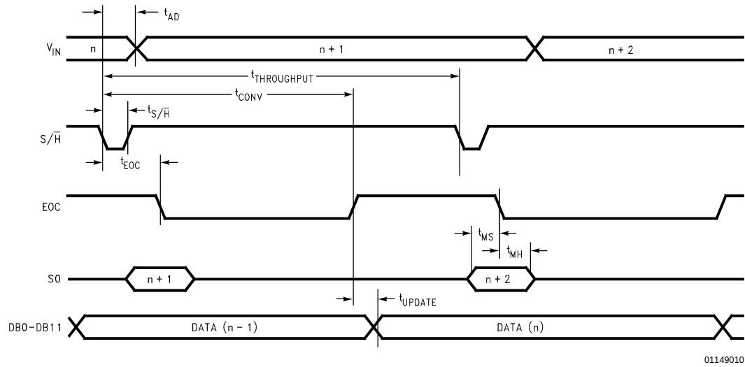
FIGURE 2. High Speed Interface Timing (MODE = 1, OE = 1, \overline{\text{CS}} = 0 , \overline{\text{RD}} = 0 )
