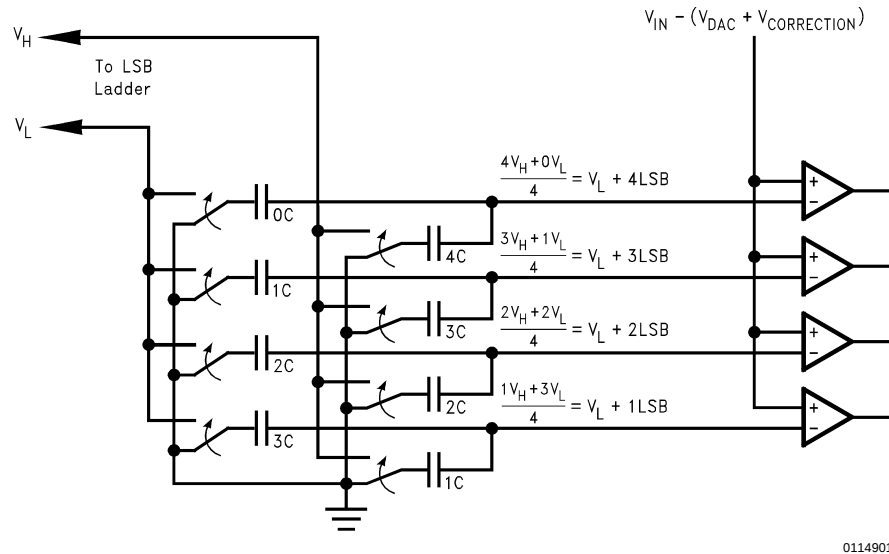
FIGURE 5. The Capacitive Voltage Divider
