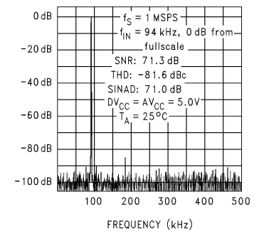
Spectral Response
