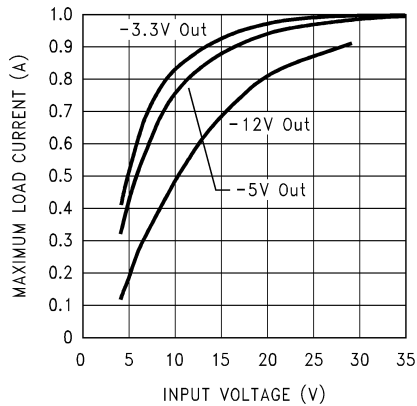
FIGURE 17. Inverting Regulator Typical Load Current
