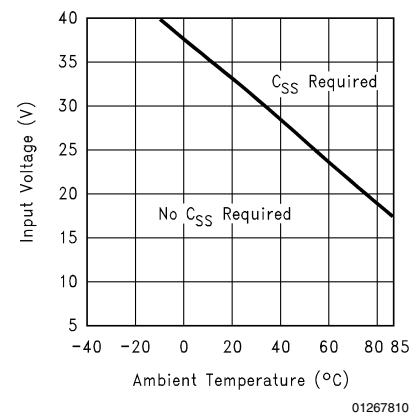
FIGURE 8. Usage of The Soft-Start Capacitor
