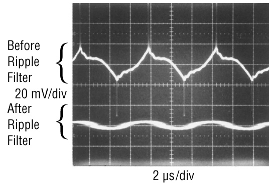
FIGURE 6. Post Ripple Filter Waveform
