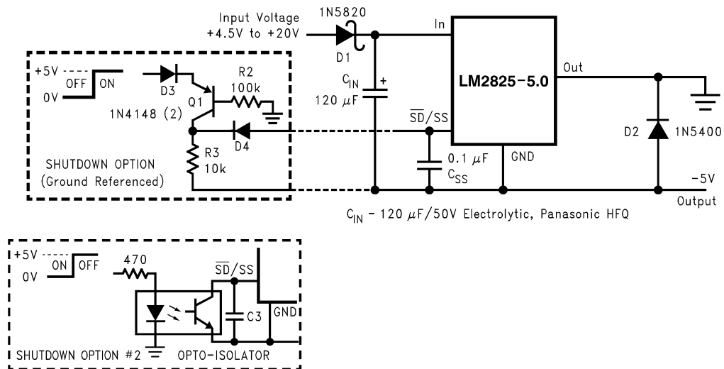
FIGURE 16. Inverting Regulator
