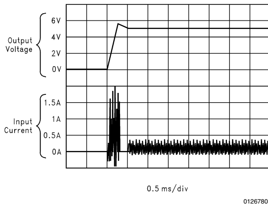
FIGURE 7. Output Voltage and Input Current during Start-Up
