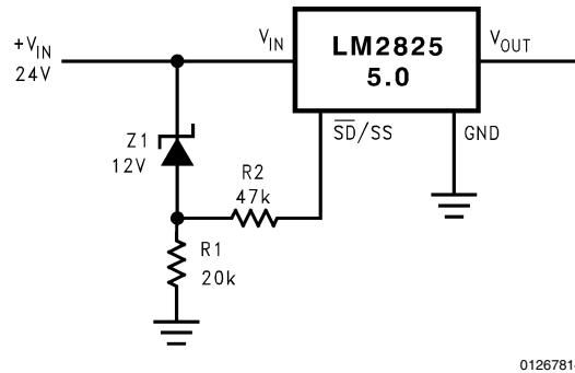
FIGURE 14. Undervoltage Lockout Circuit
