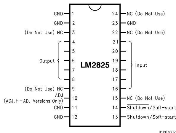
FIGURE 1. Connection Diagram
