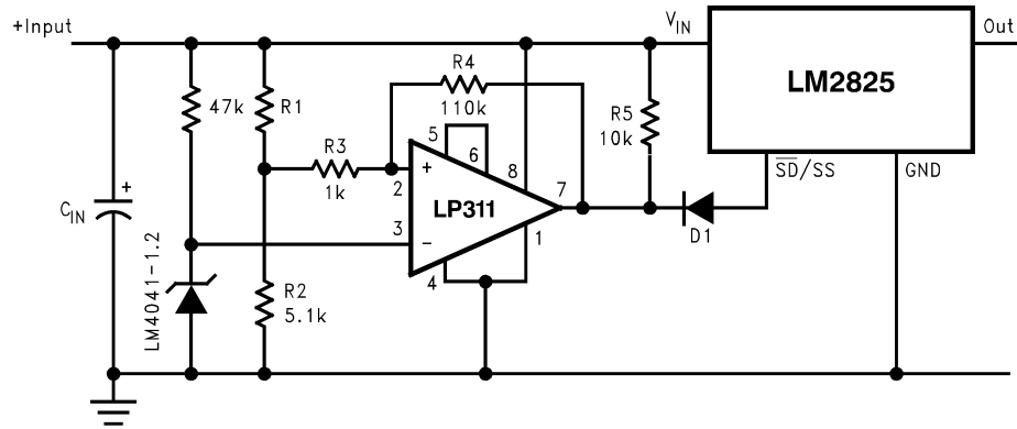
FIGURE 15. Precision Undervoltage Lockout Circuit
