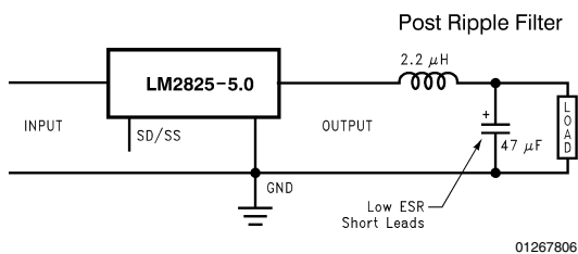
FIGURE 5. Post Ripple Filter
