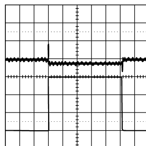
1.5A Load Transient (Sinking)
