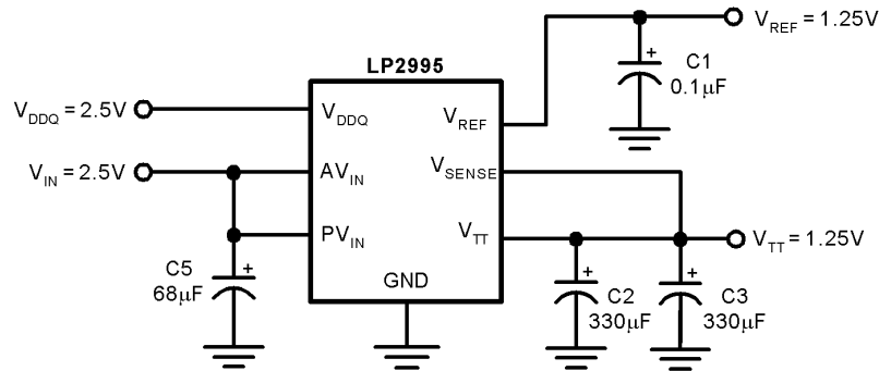
FIGURE 1. Schematic
