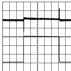
1.5A Load Transient (Sourcing)
