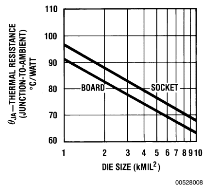
FIGURE 9. Thermal Resistance vs Board or Socket Mount
