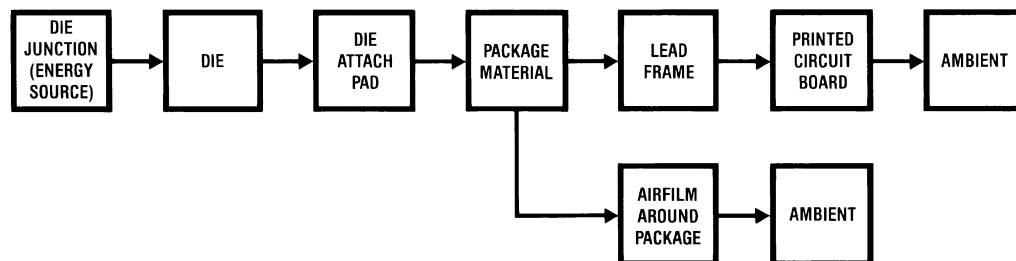
FIGURE 4. Thermal Flow (Predominant Paths)
