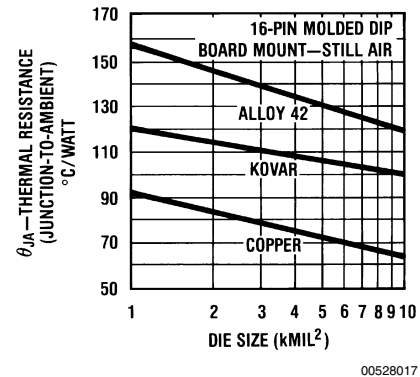
FIGURE 8. Thermal Resistance vs Lead Frame Material
