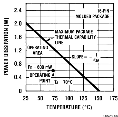
FIGURE 5. Package Power Capability vs Temperature
