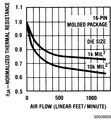
FIGURE 11. Thermal Resistance vs Air Flow (16-pin DIP)
