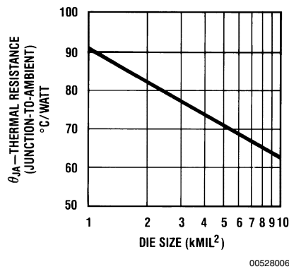
FIGURE 6. Thermal Resistance vs Die Size
