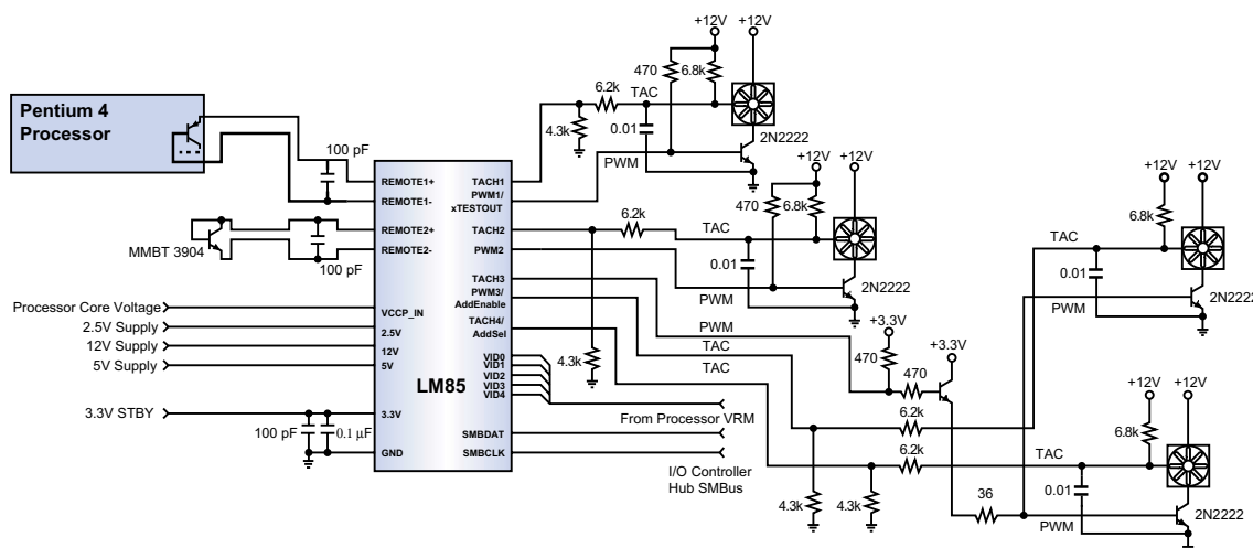
Figure 1: Typical LM85 Connection
