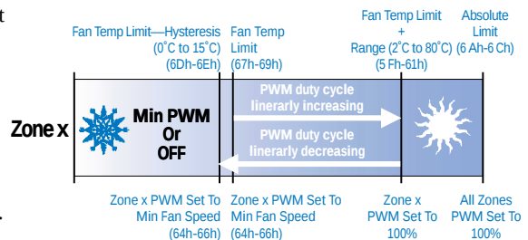
Figure 3: LM85 Fan Control Registers
