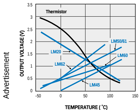
Figure 1. Comparison of analog temperature sensors to thermistors
