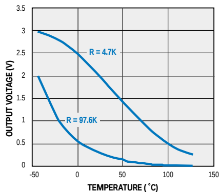
Figure 3. Thermistor output voltage vs temperature for different values of R
