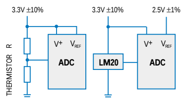
Figure 2. Connecting a thermistor or an LM20 to an ADC
