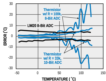
Figure 4. Comparison of Thermistor to LM20 System Performance
