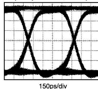
Output Eye Pattern, 1.4Gbps
