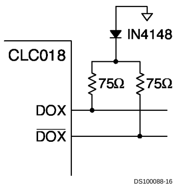
FIGURE 7. Generating 10k ECL Outputs
