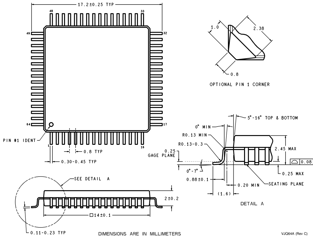
64-Lead PQFP Order Number CLC018AJVJQ NS Package Number VJQ64A
