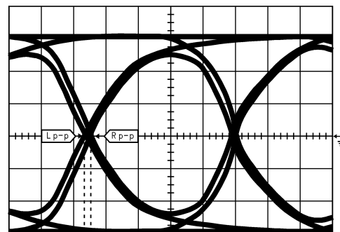
FIGURE 10. 1.485 Gbps Eye Pattern
