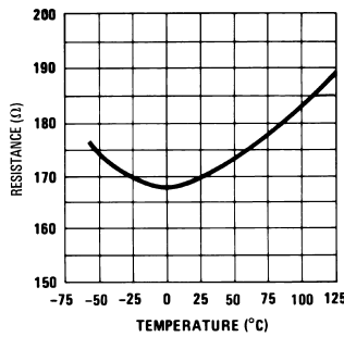
Termination Resistance
