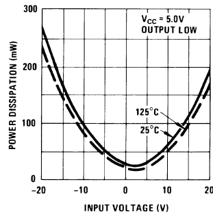
Internal Power Dissipation
