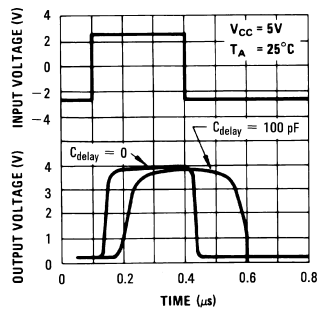
Response Time
