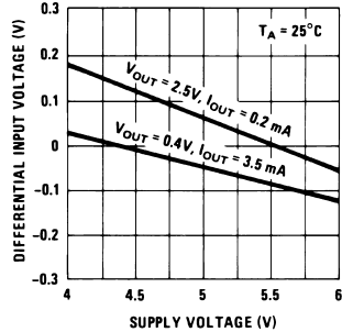
Supply Voltage Sensitivity
