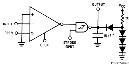
Differential and Strobe Input Signal
