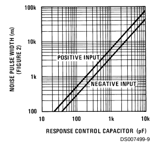
FIGURE 1. Noise Pulse Width vs Response Control Capacitor
