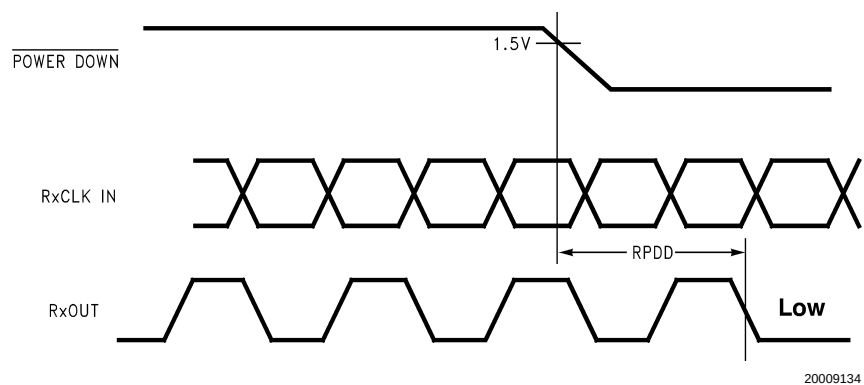
FIGURE 12. DS90CR482 (Receiver) Power Down Delay
