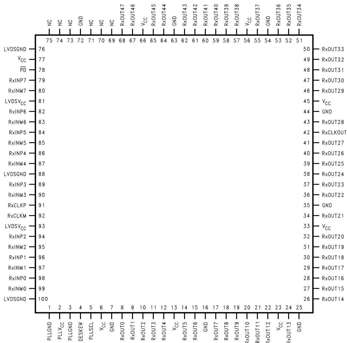
Receiver - DS90CR482 - TQFP - Top View
