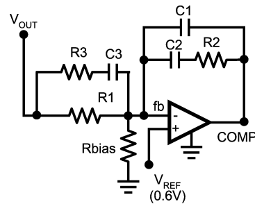
FIGURE 15. Type 3 Compensation
