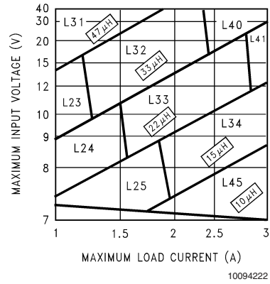
FIGURE 4. LM2670-5.0
