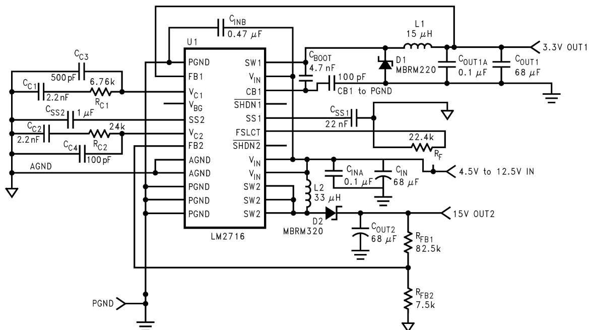
FIGURE 3. 15V, 3.3V Output Application
